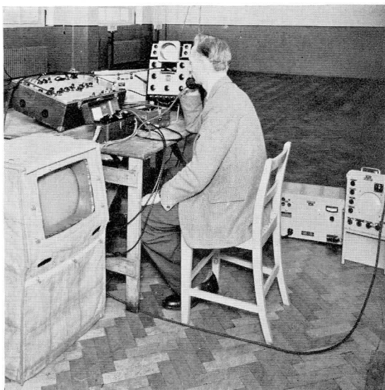
Fig. 4: Intermediate video repeater point at Cardiff automatic telephone exchange
