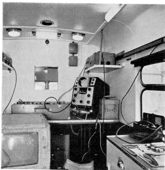
Fig. 2: Mobile repeater station—internal view showing video repeater equipment
