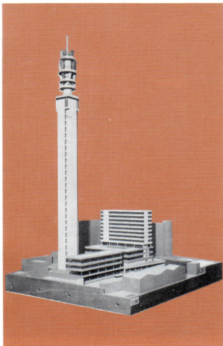
Initially, four paths will radiate from the London Tower, one of them toward the great industrial regions of the Midlands and North via this Tower at Birmingham.
